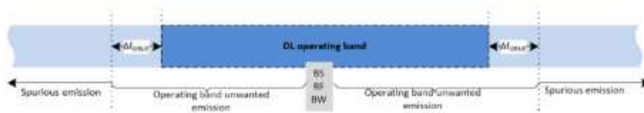
Gambar 5. Definisi Unwanted Emission
