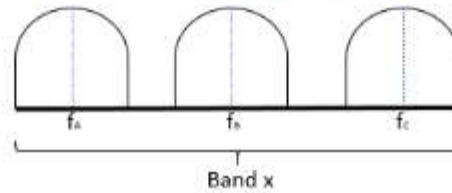
Gambar 2. Intraband non-Contiguous .
