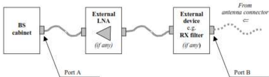
Gambar 2. Interface penerima BS type 1-C.
