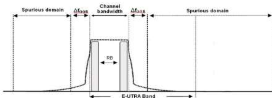
Gambar 2. Spektrum Transmitter.
